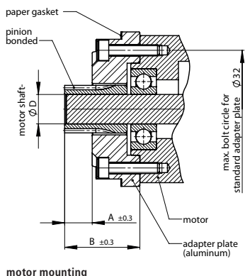
motor mounting
